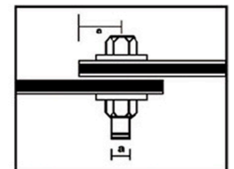
Clamping & Bolting
